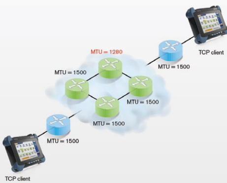
Figure 15. Path MTU discovery
