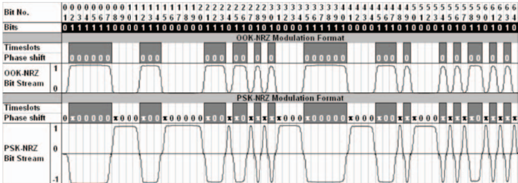
Diagram 20 – Phase-shift keying applied to NRZ bit stream
