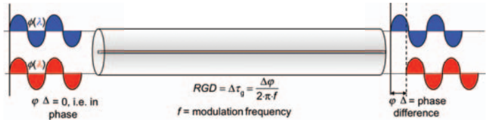
Diagram 27 – Measurement basis of the phase-shift method
