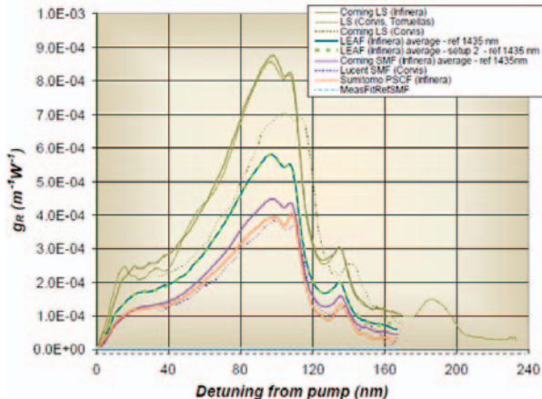
Diagram 40 – Raman gain with respect to fiber type
