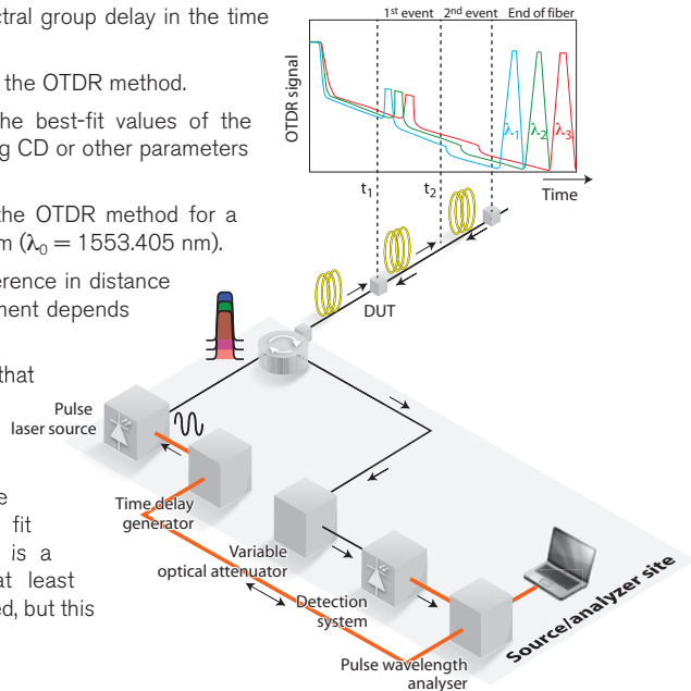
Diagram 36 – Operating principle of the OTDR method
