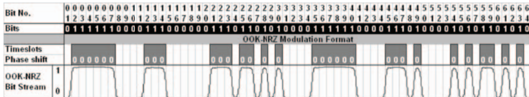
Diagram 16 – Example of NRZ format transmission
