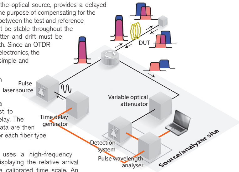
Schematic of the OTDR setup
